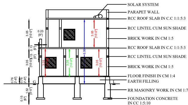
SECTION "AA","BB"
