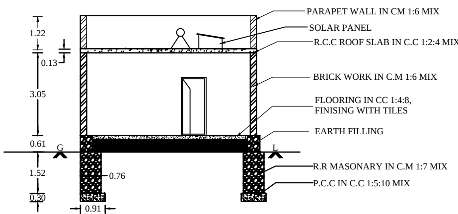
SECTION "A-B"
