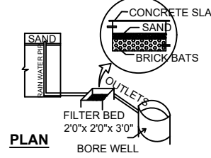
RAIN WATER HARVEST SYSTEM (NOT TO SCALE)
