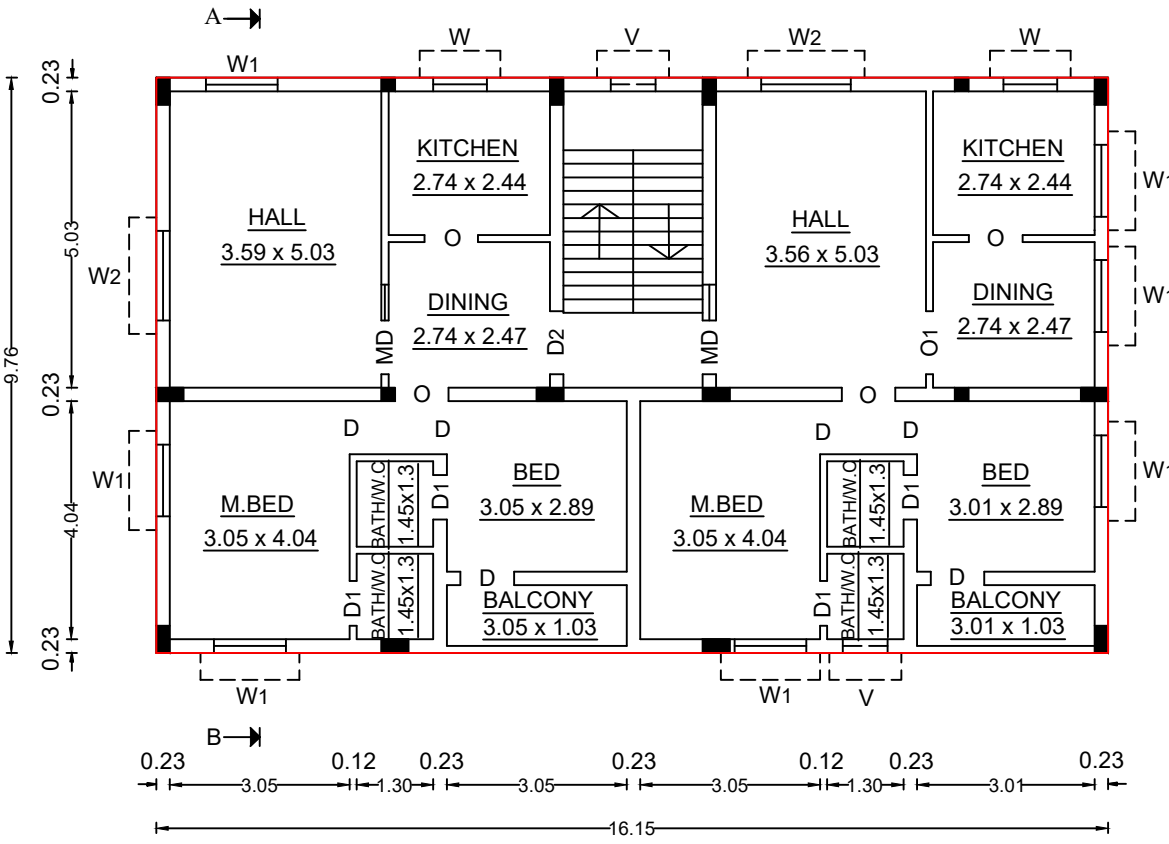
FIRST FLOOR PLAN (WEST FACING)
