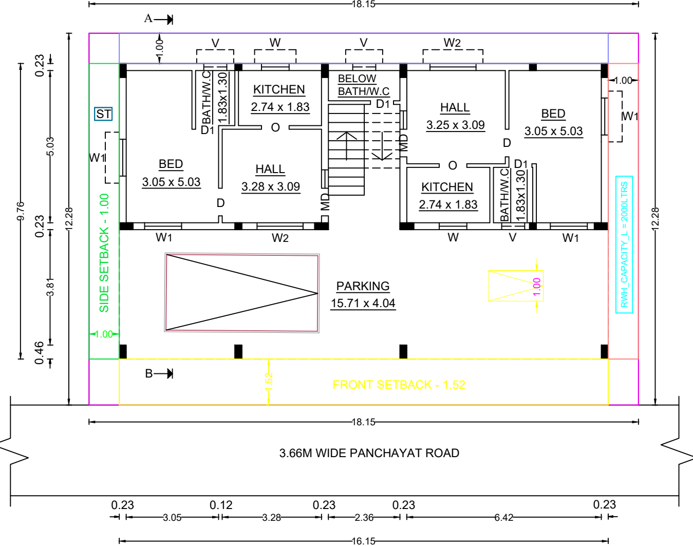
GROUND FLOOR PLAN (WEST FACING)
