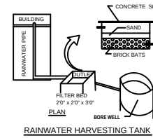
RAINWATER HARVESTING TANK
