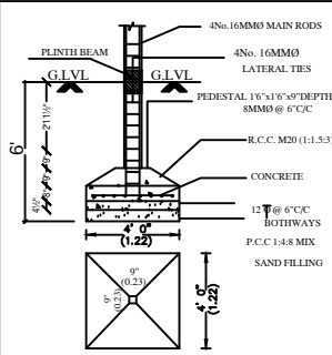
FOUNDATION DETAIL
