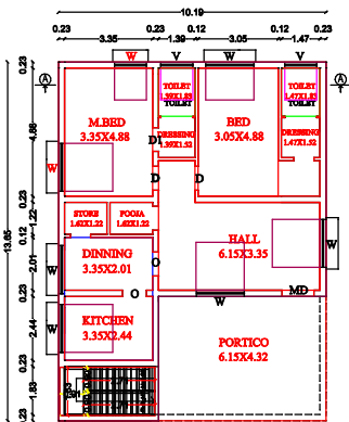
PRO. GROUND FLOOR
