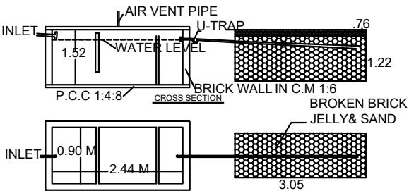
SEPTIC TANK (NOT TO SCALE)
