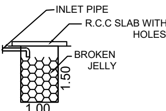
RAIN WATER HARVESTING FILTER BED
