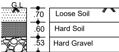
TRIAL PIT DETAILS (NOT TO SCALE)
