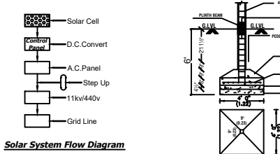
Solar System Flow Diagram
