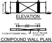
COMPOUND WALL PLAN
