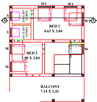
LOOR PLAN
