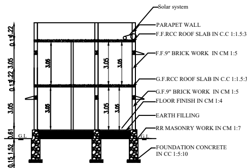
SECTION ON AA & BB
