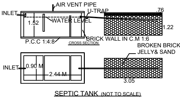
SEPTIC TANK (NOT TO SCALE)
