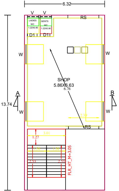
GROUND FLOOR PLAN SCALE 1 CM = 1 M
