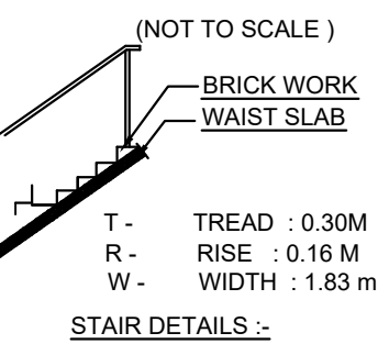
STAIR DETAILS :-
