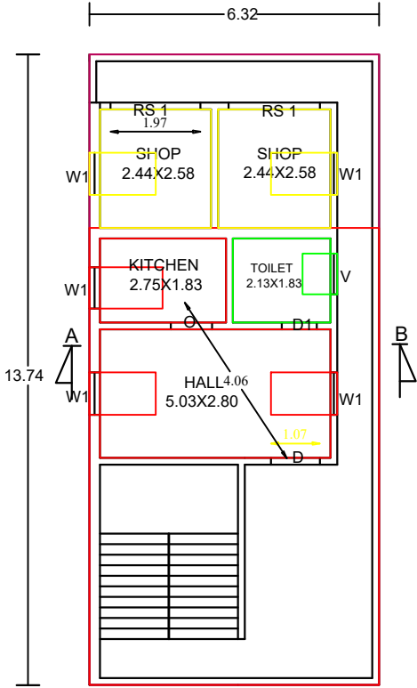
FRIST FLOOR PLAN SCALE 1 CM = 1 M
