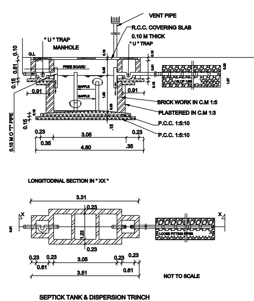
SEPTIC TANK & DISPERSION TRENCH
