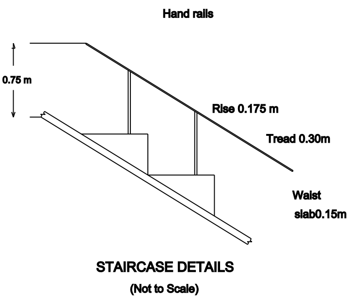
STAIRCASE DETAILS (Not to Scale)
