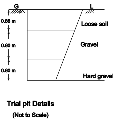
Trial pit Details (Not to Scale)
