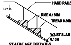
STAIRCASE DETAILS
