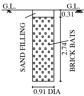
RAINWATER COLLECTION PIT PERCUATION AND DETAILED PLAN
