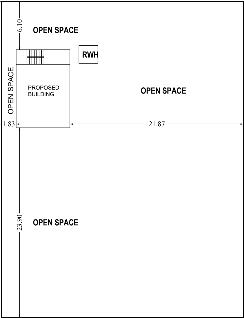
RAINWATER COLLECTION PIT PERCUATION AND DETAILED PLAN
