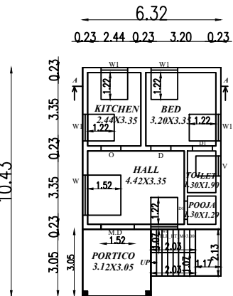
GROUND FLOOR PLAN (SCALE 1:100)
