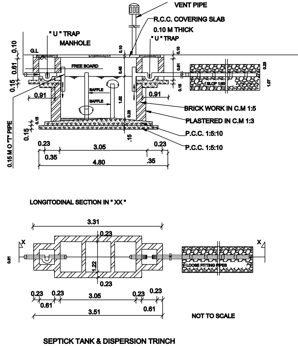
SEPTICK TANK & DISPERSION TRINCH
