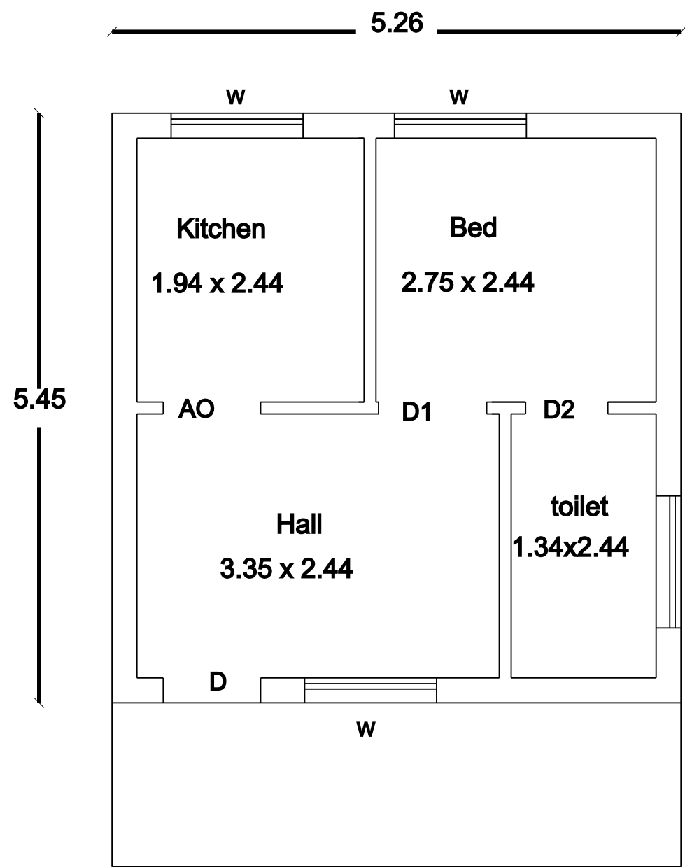
Plan
