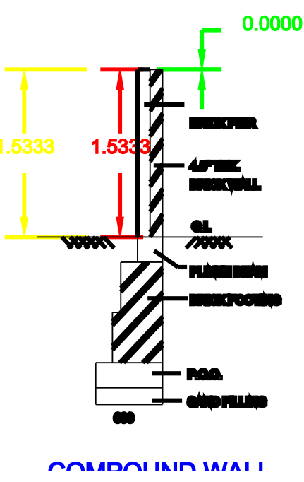
COMPOUND WALL
