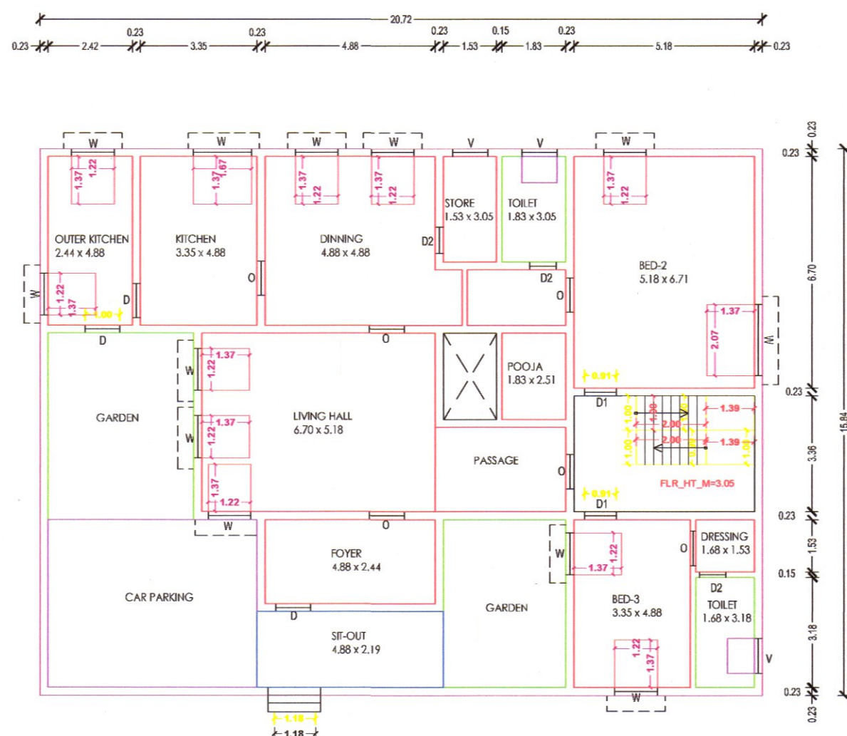
GROUND FLOOR PLAN (BLOCK - 1 - PROPOSED RESIDENTIAL BUILDING)
