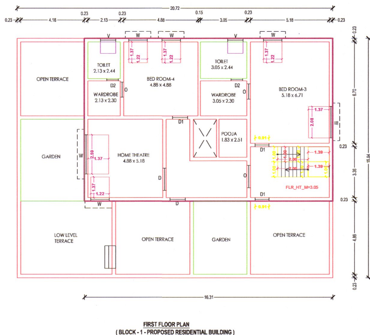
FIRST FLOOR PLAN (BLOCK - 1 - PROPOSED RESIDENTIAL BUILDING)
