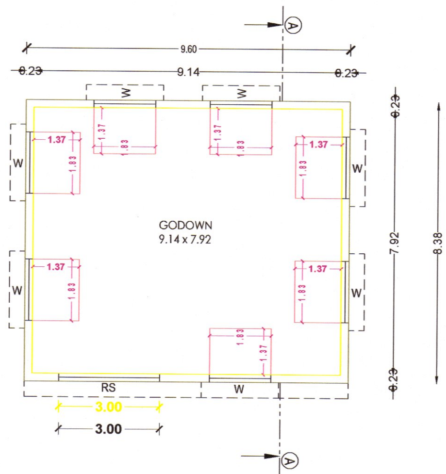
GROUND FLOOR PLAN (BLOCK - 1 - PROPOSED COMMERCIAL BUILDING)
