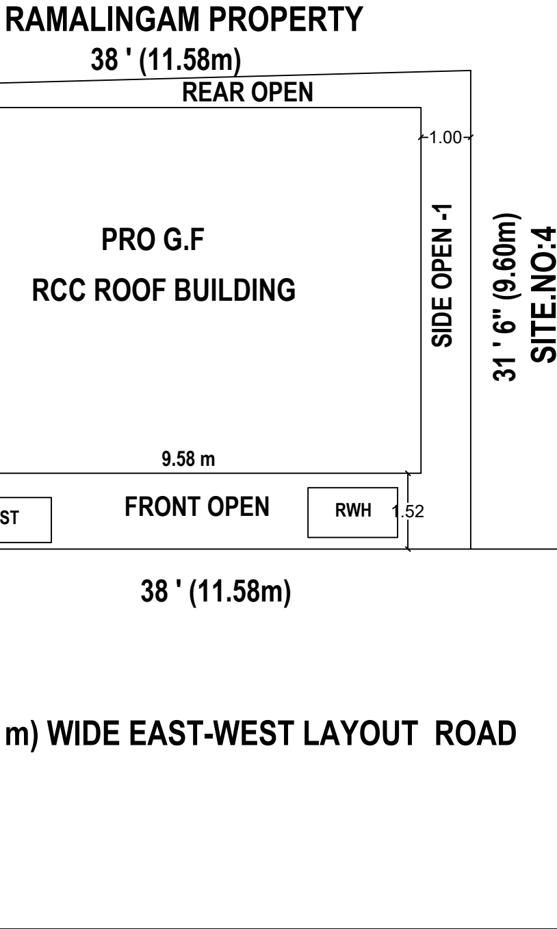
SITE PLAN
