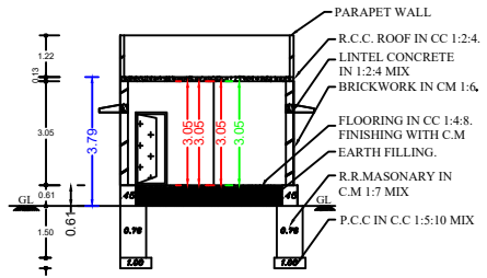
SECTION HK'
