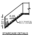
STAIRCASE DETAILS
