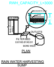
RAIN WATER HARVESTING SUMP
