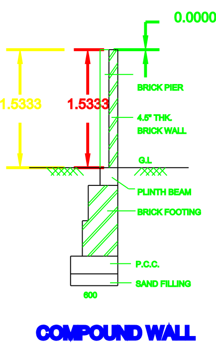
COMPOUND WALL
