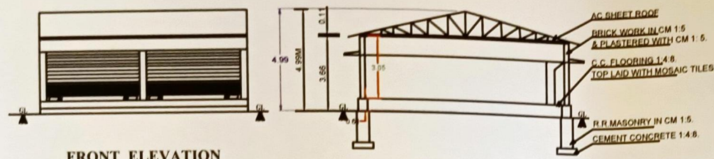
SECTION "A-B"
