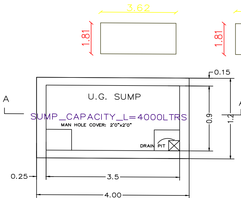
PLAN OF SUMP DETAIL SCALE 1"=4'0"
