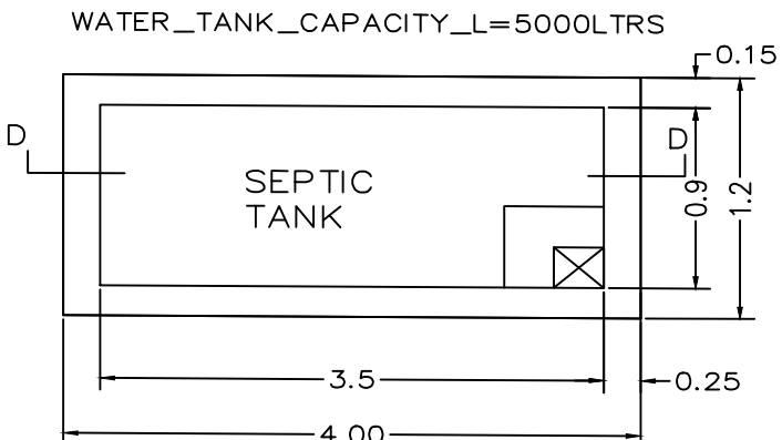
PLAN OF SEPTIC TANK SCALE 1"=2'0"
