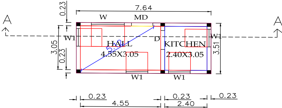
GROUND FLOOR
