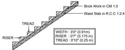
STAIRCASE DETAILS
