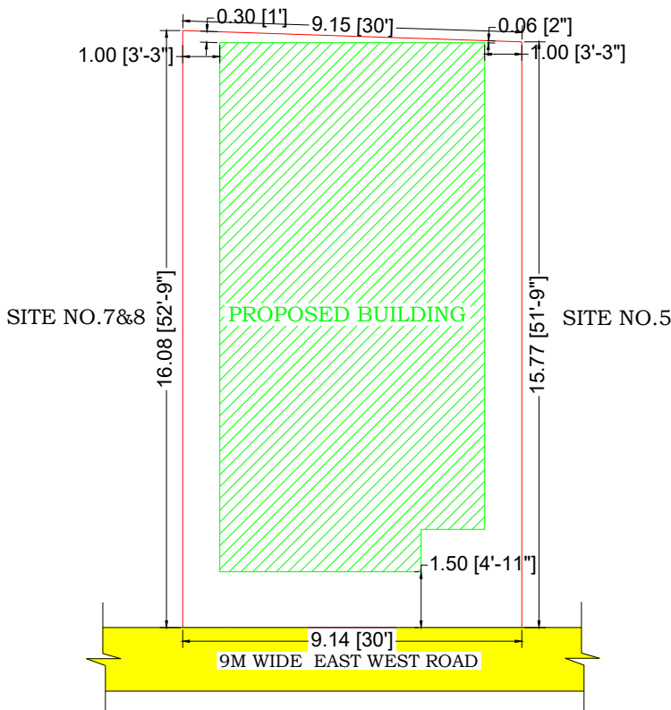
SITE PLAN
