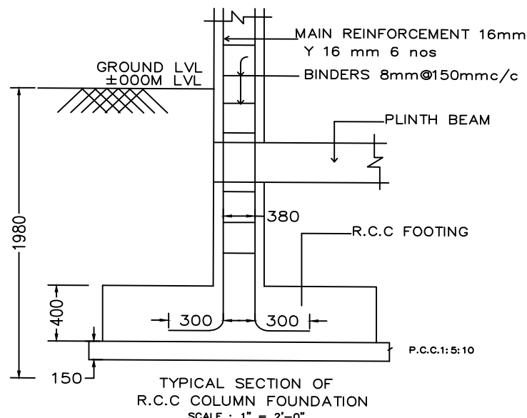
TYPICAL SECTION OF R.C.C COLUMN FOUNDATION SCALE : 1" = 2'-0"
