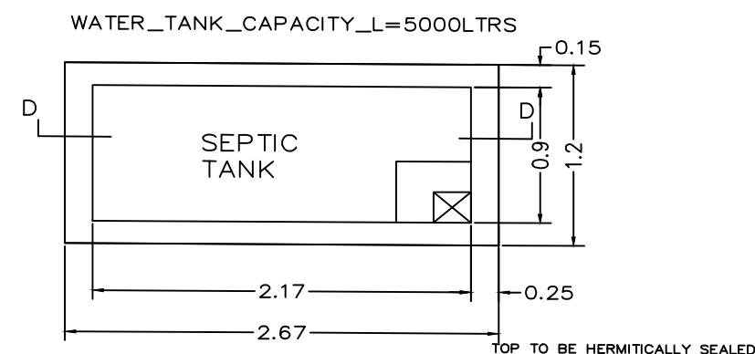
PLAN OF SEPTIC TANK SCALE 1"=2'0"
