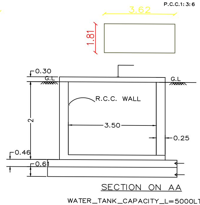
SECTION ON AA WATER_TANK_CAPACITY_L=5000LTRS
