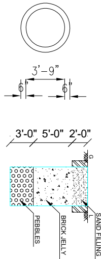
RAINWATER HARVESTING
