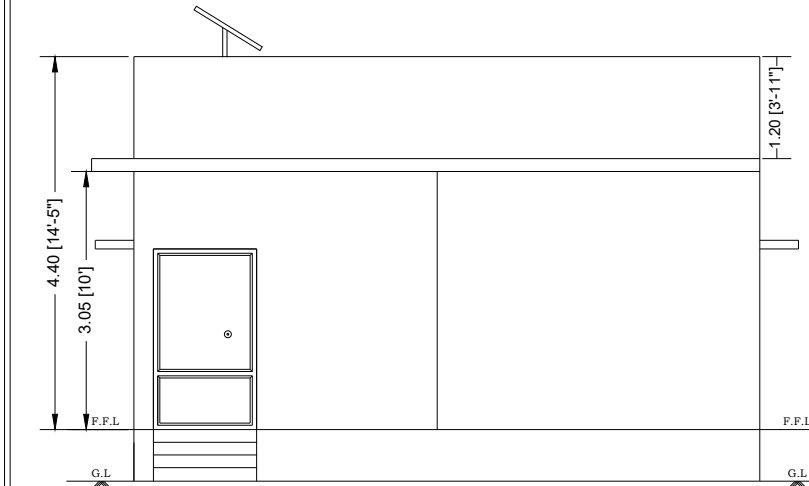
FRONT ELEVATION
