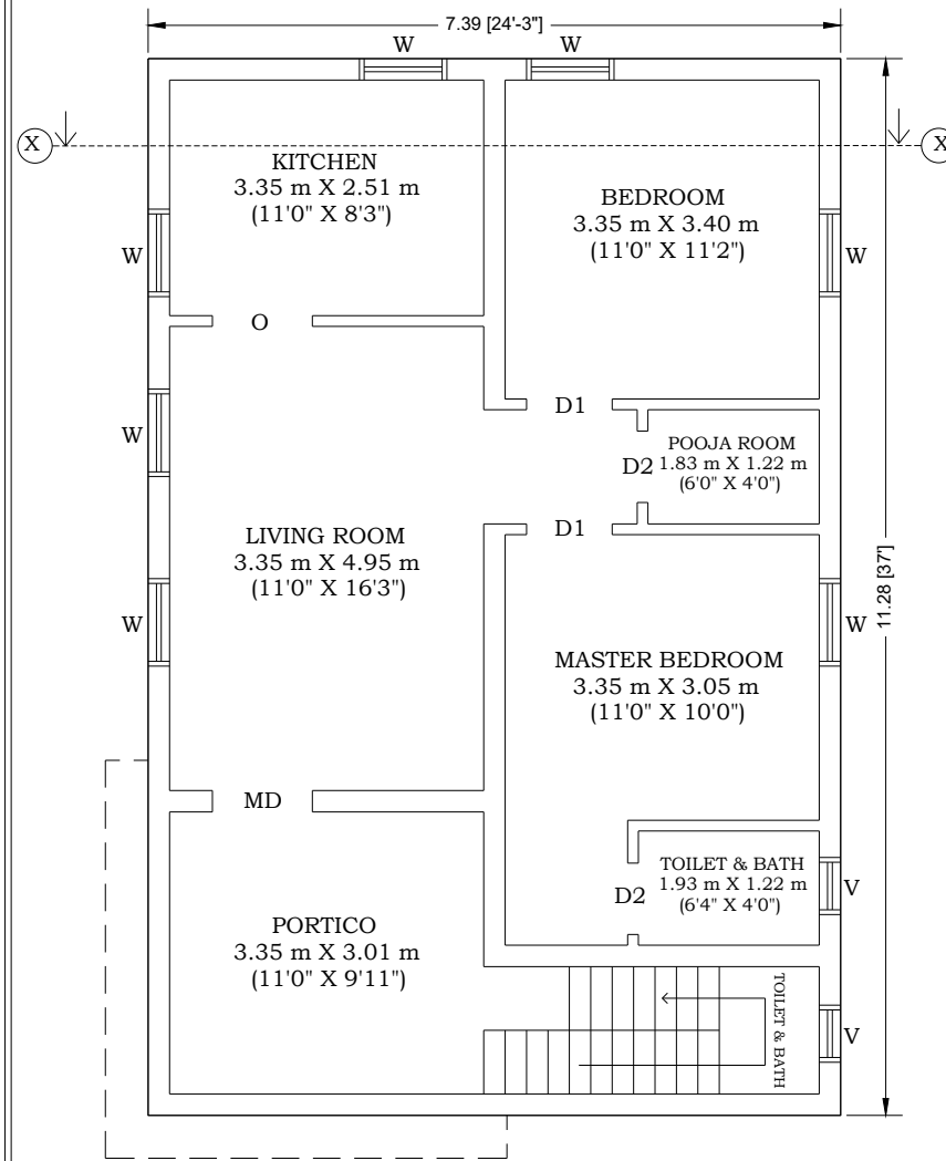
GROUND FLOOR
