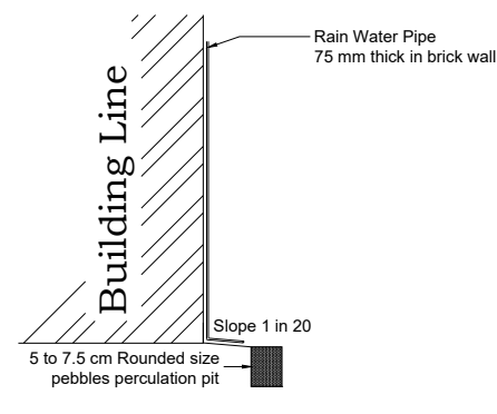
RAINWATER HARVESTING
