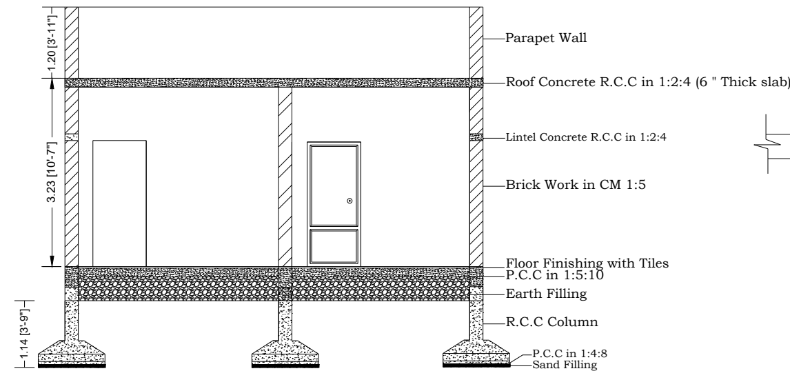
SECTION X-X
