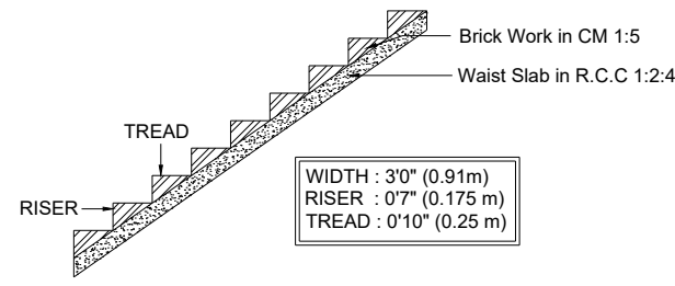
STAIRCASE DETAILS
