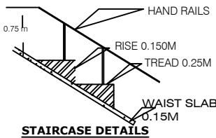
STAIRCASE DETAILS
