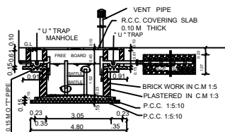
SEPTICK TANK & DISPERSION TRINCH
