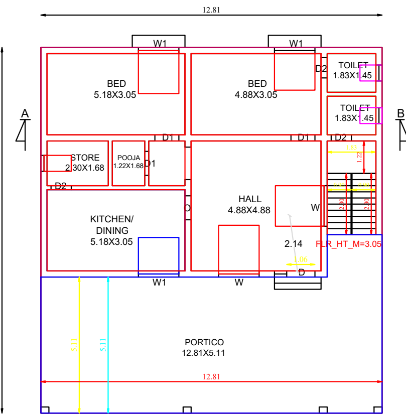
GROUND FLOOR PLAN SCALE 1 CM = 1 M
