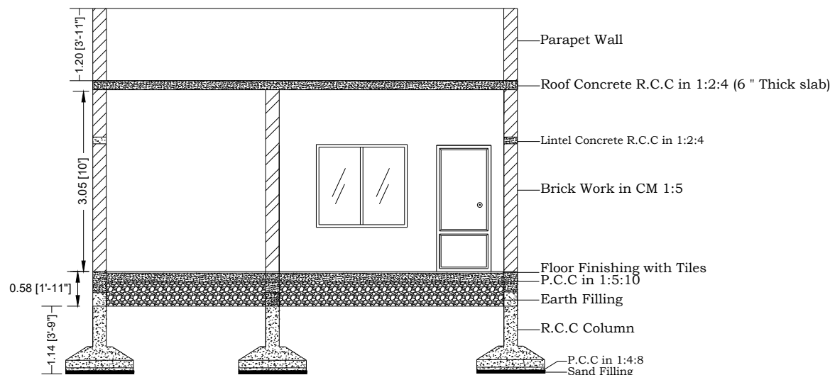
SECTION X-X
