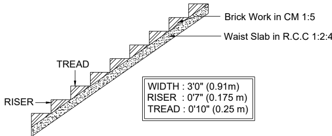
STAIRCASE DETAILS
