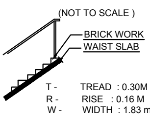
STAIR DETAILS :-
