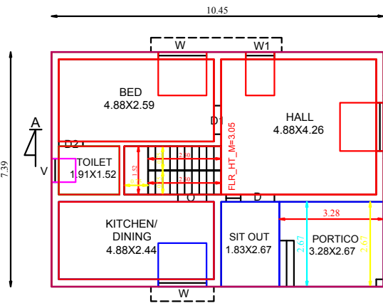
GROUND FLOOR PLAN SCALE 1 CM = 1 M
