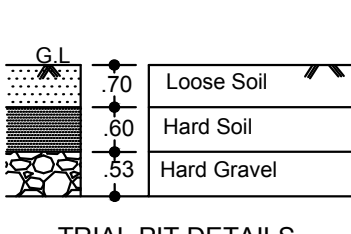
TRIAL PIT DETAILS (NOT TO SCALE)
