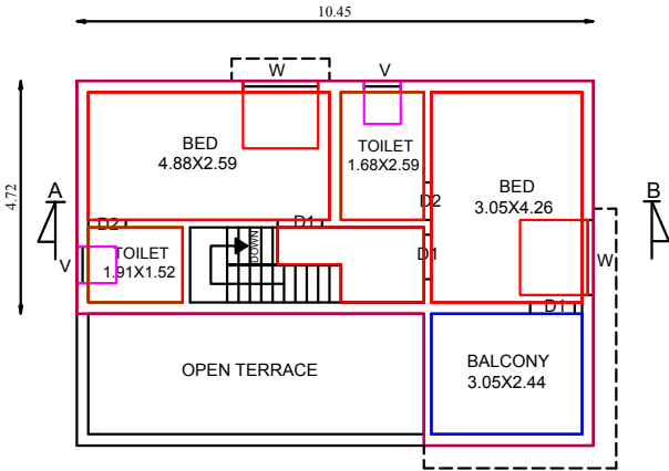
FIRST FLOOR PLAN SCALE 1 CM = 1 M
