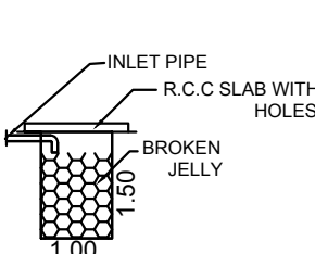
RAIN WATER HARVESTING FILTER BED
