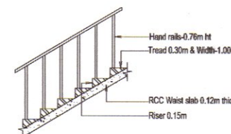
STAIRCASE DETAILS
