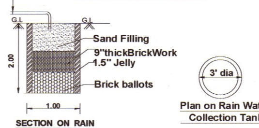
RAIN WATER COLLECTION TANK
