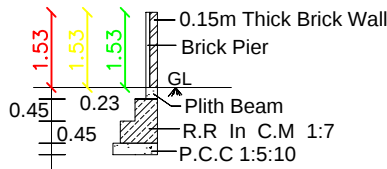
COMPOUND WALL DETAILS
