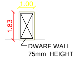
WICKET GATE
