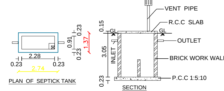
SEPTIC TANK DETAILS
