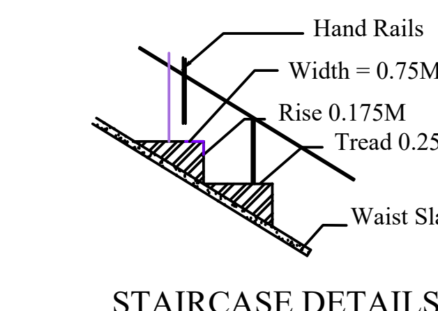
STAIRCASE DETAILS
