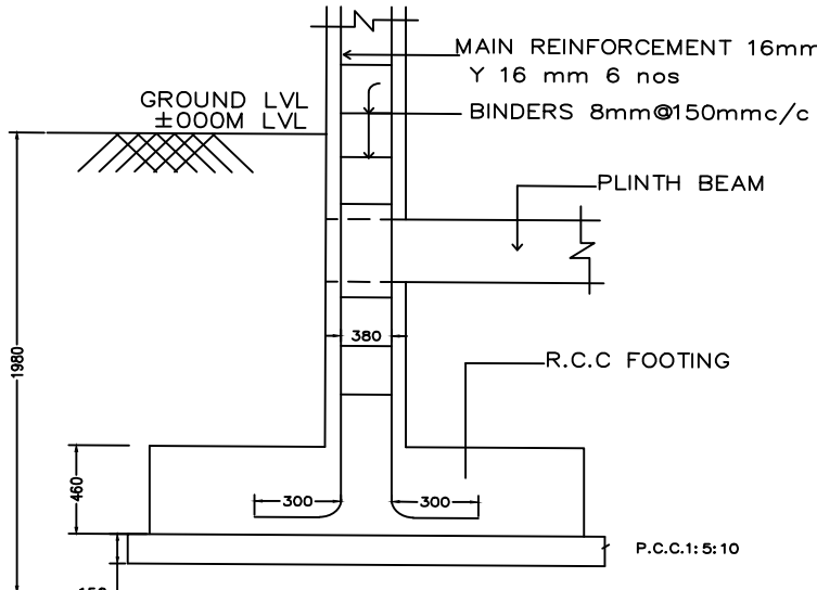
TYPICAL SECTION OF R.C.C COLUMN FOUNDATION SCALE : 1" = 2'-0"
