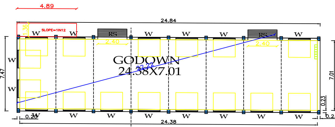
GROUND FLOOR
