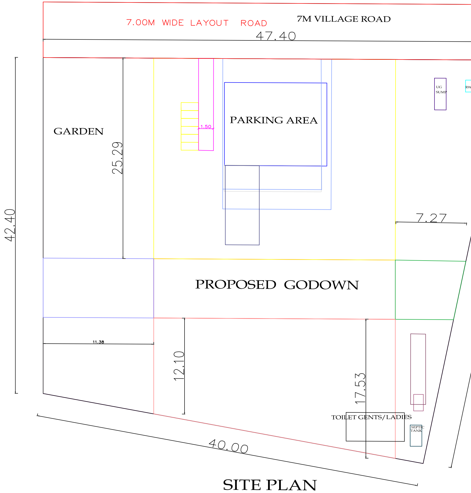
SITE PLAN
