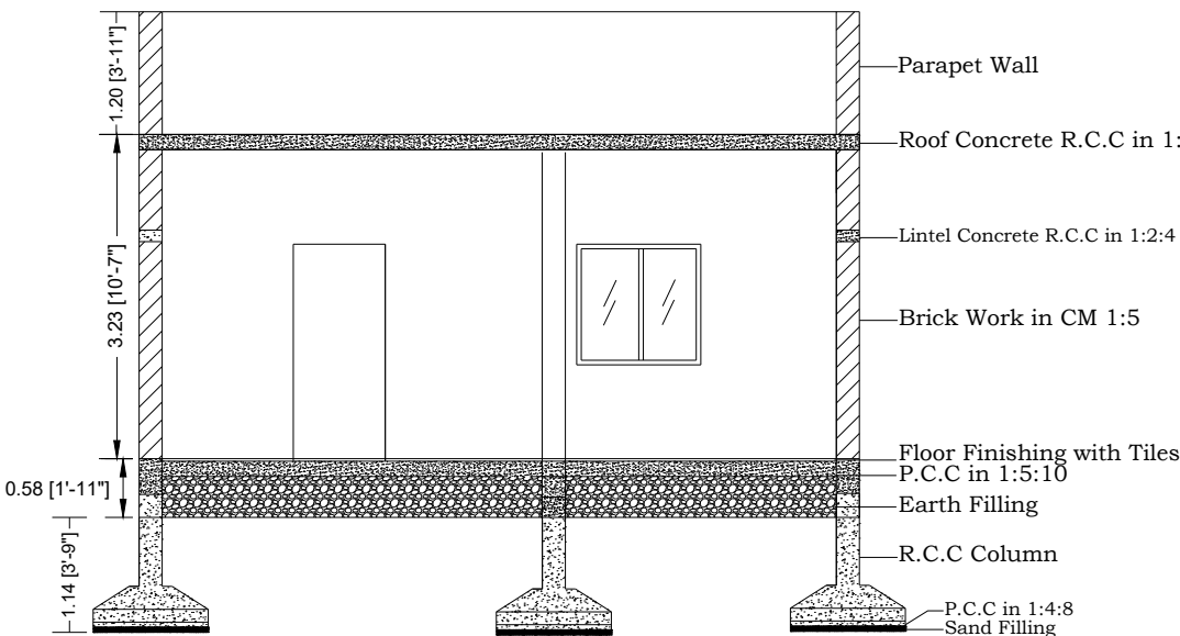
SECTION X-X
