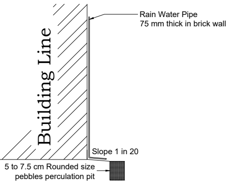
RAINWATER HARVESTING
