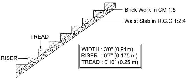
STAIRCASE DETAILS
