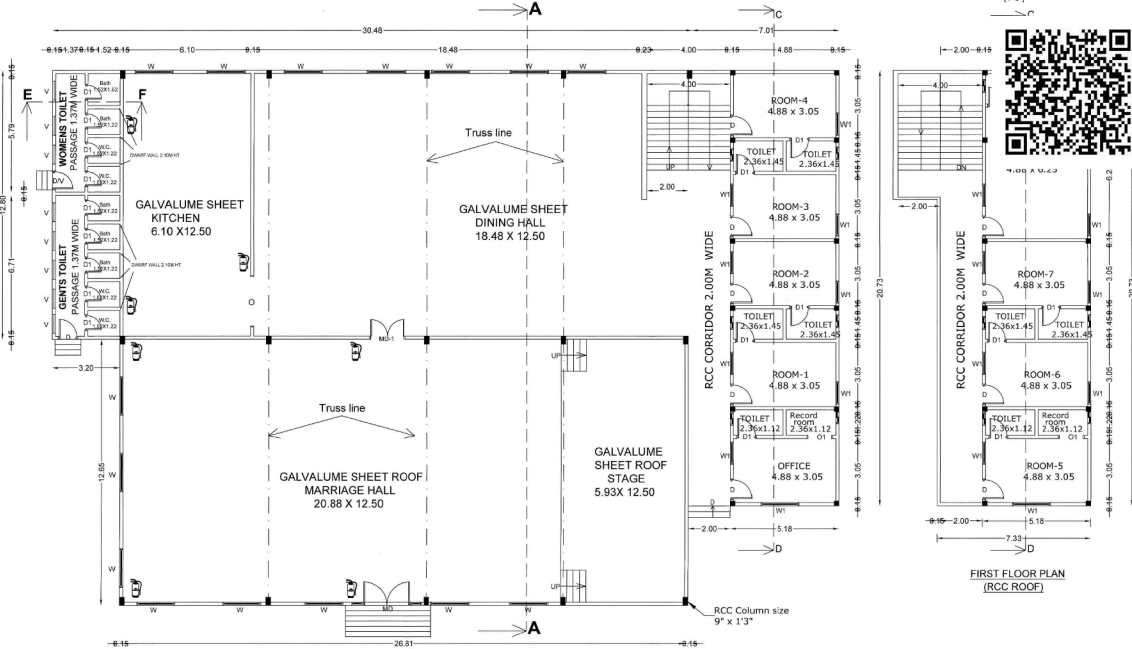
GROUND FLOOR PLAN (GALVALUME SHEET ROOF & R.C.C. ROOF)
