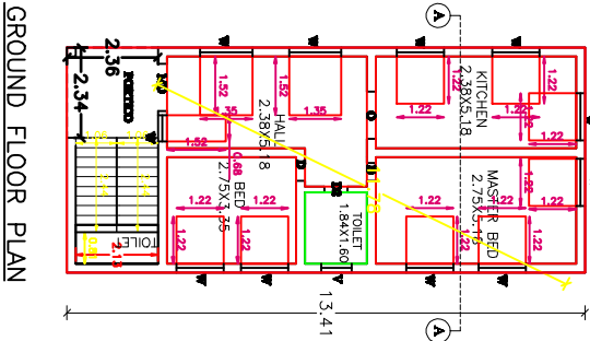
DETAILED PLAN: SCALE 1:100
