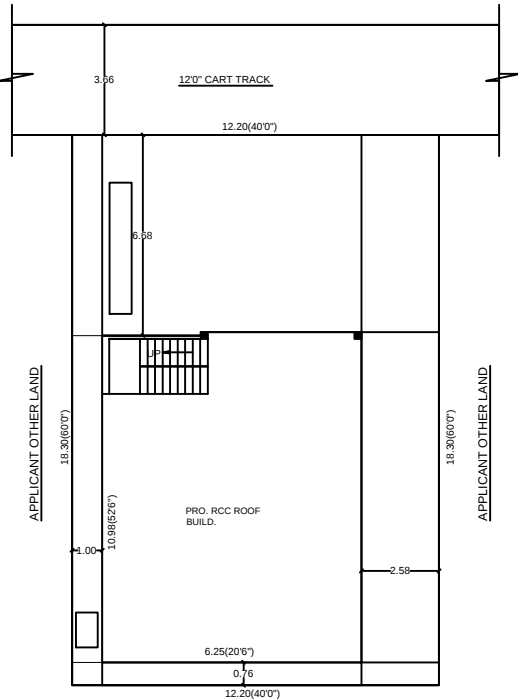
APPLICANT OTHER LAND SITE PLAN
