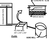
RAINWATER HARVESTING TANK
