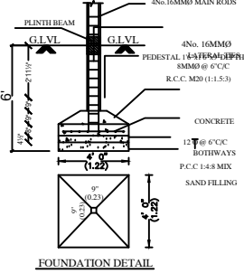
FOUNDATION DETAIL
