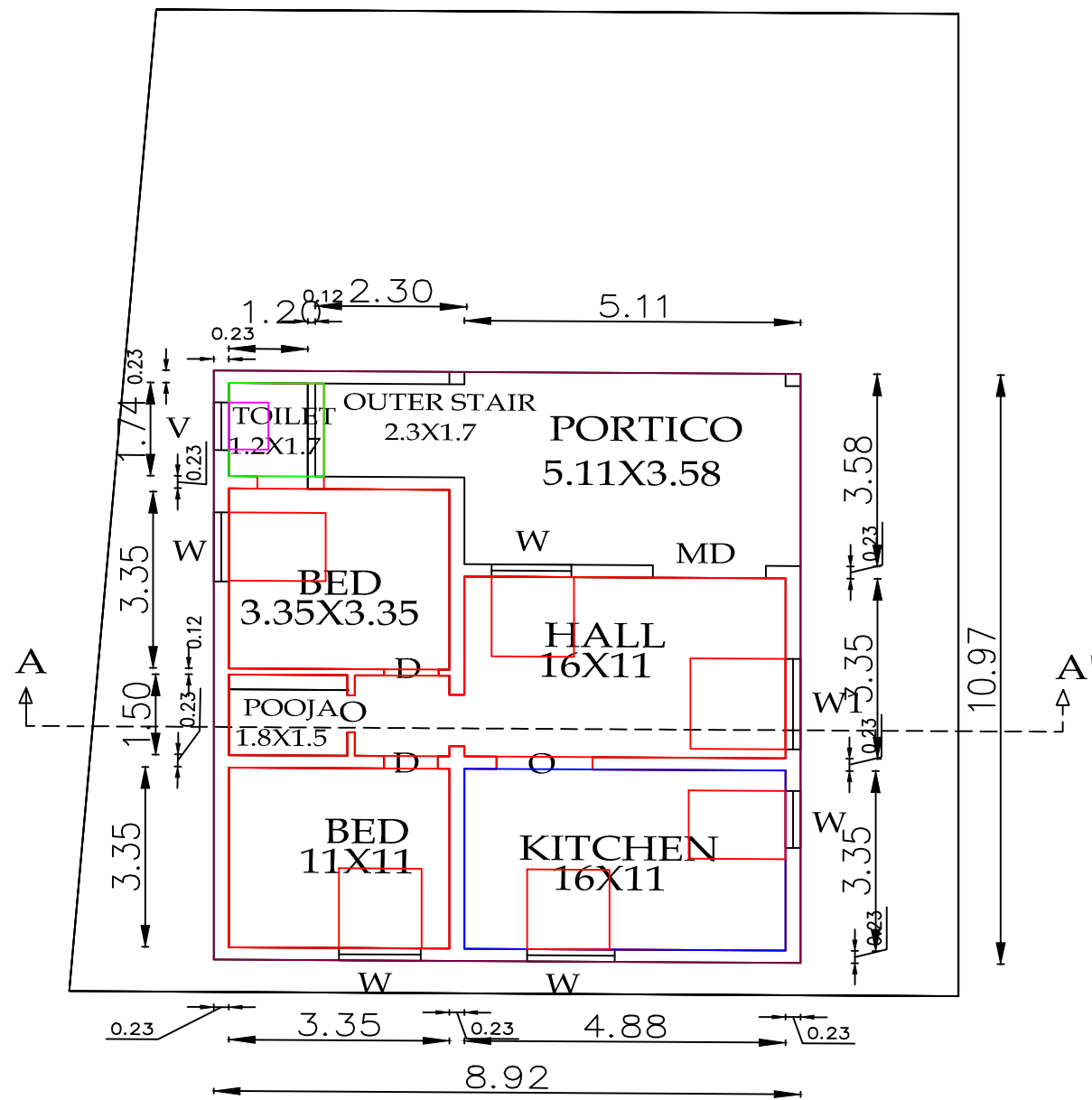
GROUND FLOOR
