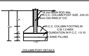
COLUMN POST DETAILS
