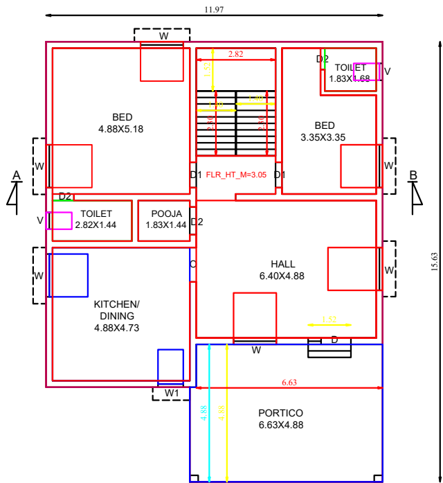
GROUND FLOOR PLAN SCALE 1 CM = 1 M
