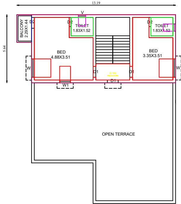
FIRST FLOOR PLAN SCALE 1 CM = 1 M
