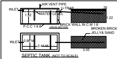
SEPTIC TANK (NOT TO SCALE)
