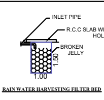
RAIN WATER HARVESTING FILTER BED
