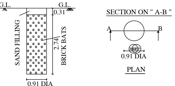
RAINWATER COLLECTION PIT PERCUATION AND DETAILED PLAN
