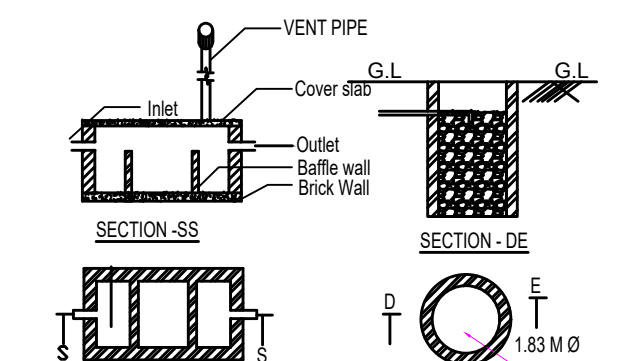
SEPTIC TANK & SOAK PIT DETAILS
