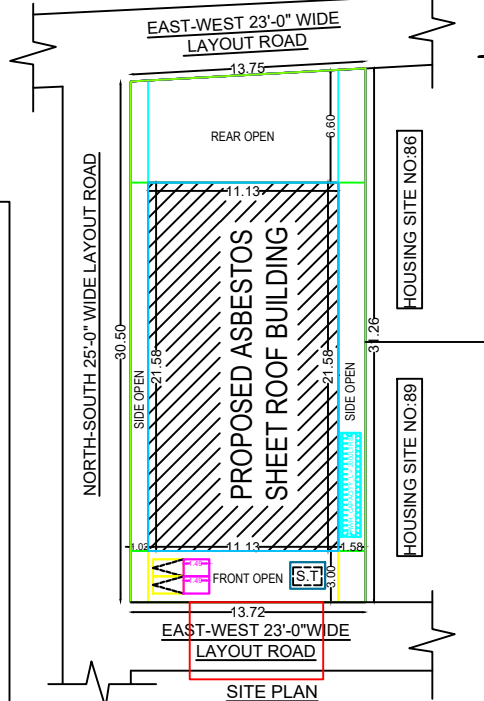
SITE PLAN
