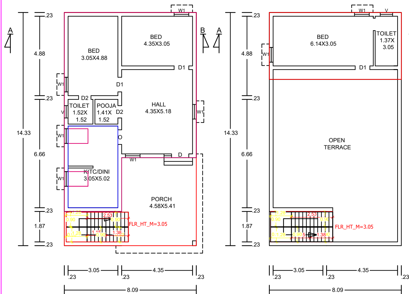
GROUND FLOOR PLAN SCALE 1 CM =1 M
