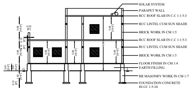
SECTION "AA" & "BB"
