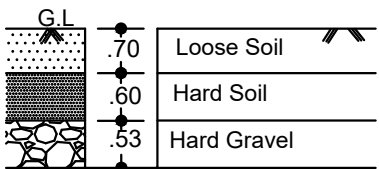
TRIAL PIT DETAILS (NOT TO SCALE)
