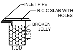
RAIN WATER HARVESTING FILTER BED
