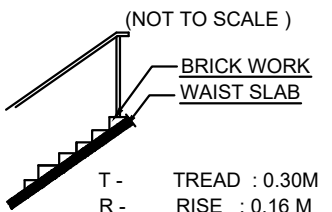
STAIR DETAILS :-
