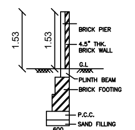
COMPOUND WALL
