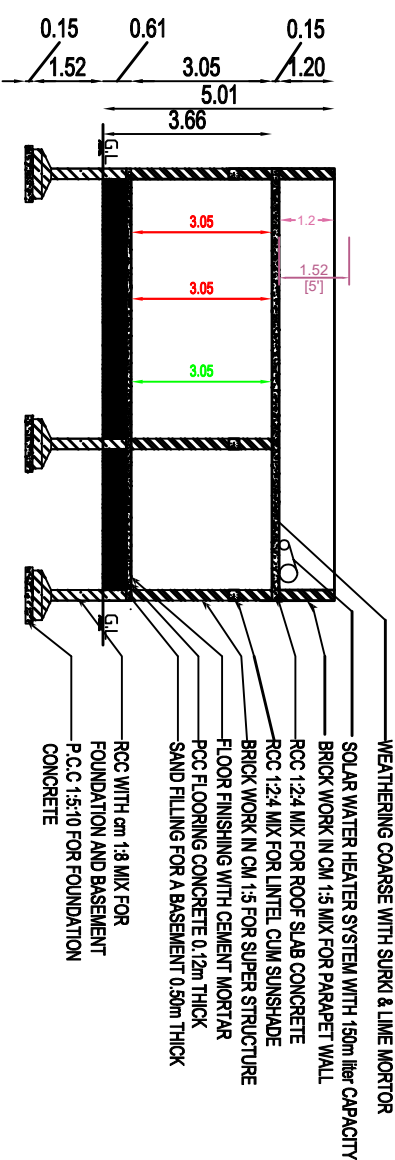
SECTION -AA
