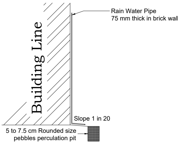
RAINWATER HARVESTING
