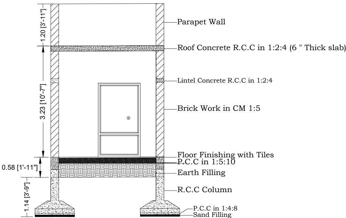
SECTION X-X
