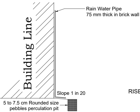
RAINWATER HARVESTING
