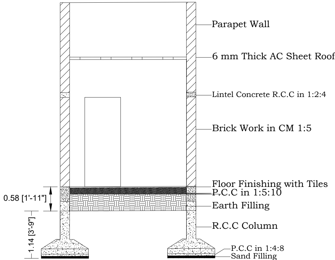
SECTION X-X
