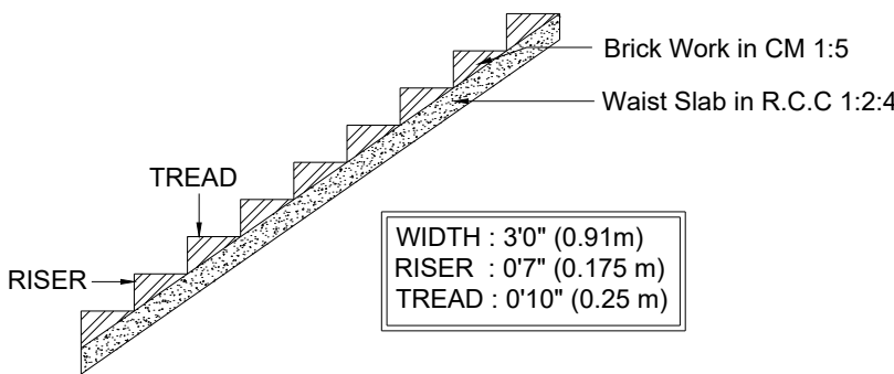
STAIRCASE DETAILS
