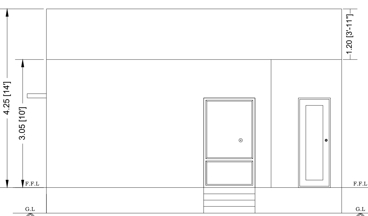
FRONT ELEVATION
